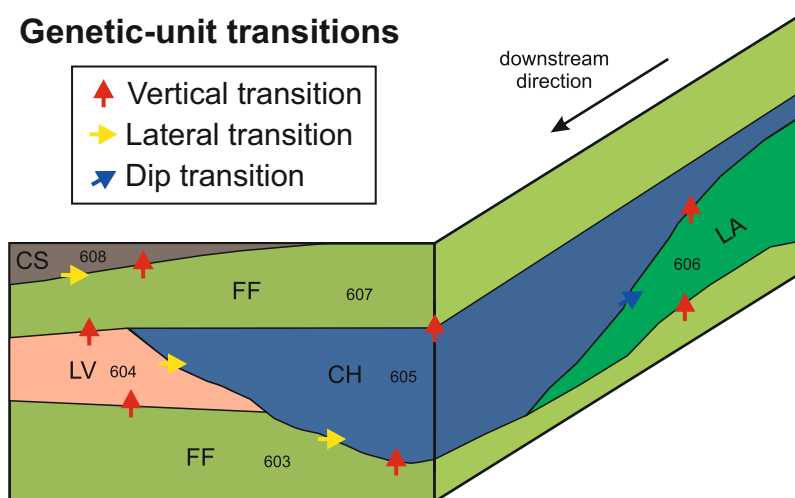
Above. Spatial relationships between units are stored in the form of transitions between pairs of units, in three dimensions (vertically, along strike, up-dip). This enables spatial relationships between architectural elements and facies units to be examined, for example to predict systematic proximal-to-distal changes.
