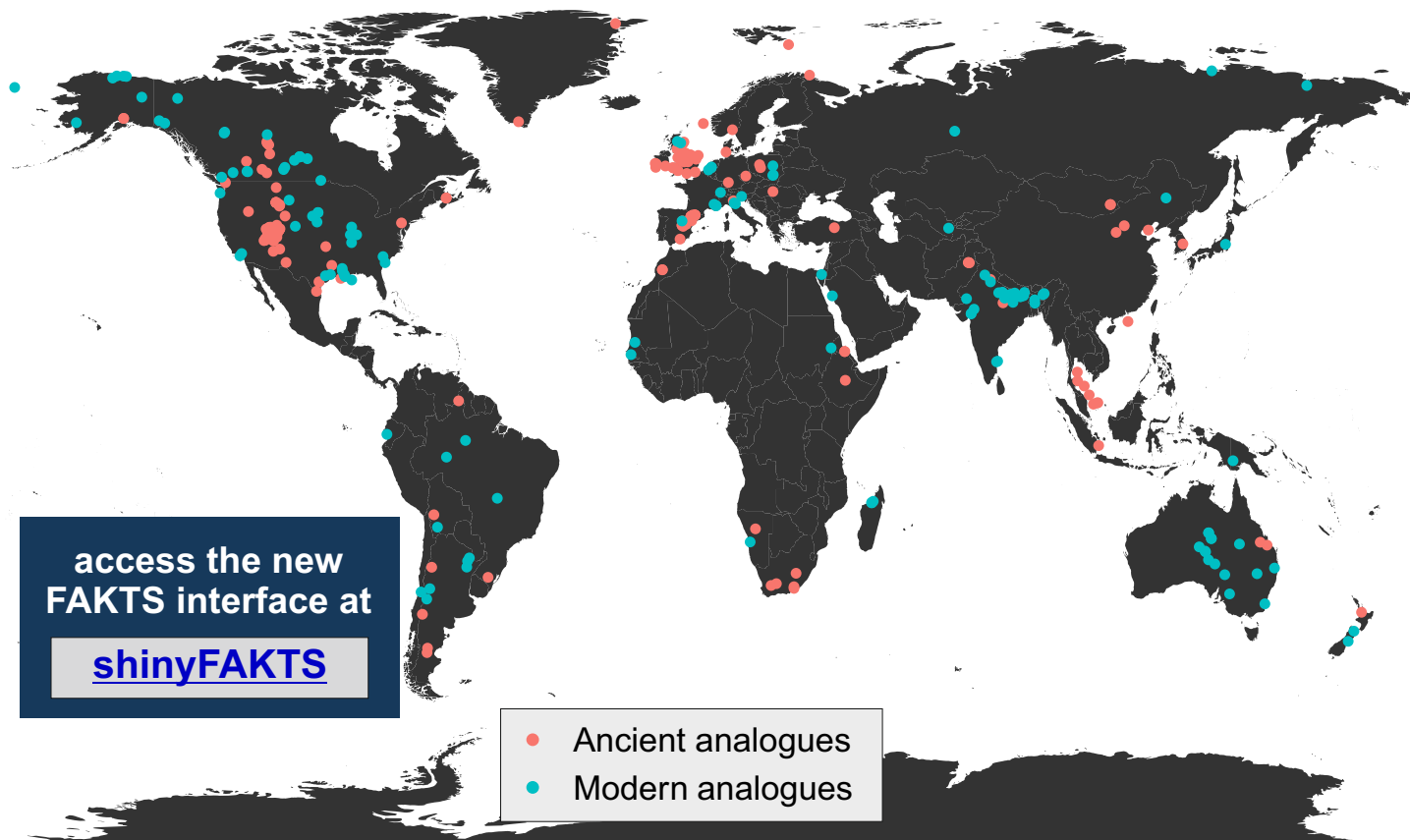
Above. Geographic distribution of some of the 349 analogue studies contained in FAKTS, as of June 2022. Database population is on-going.
