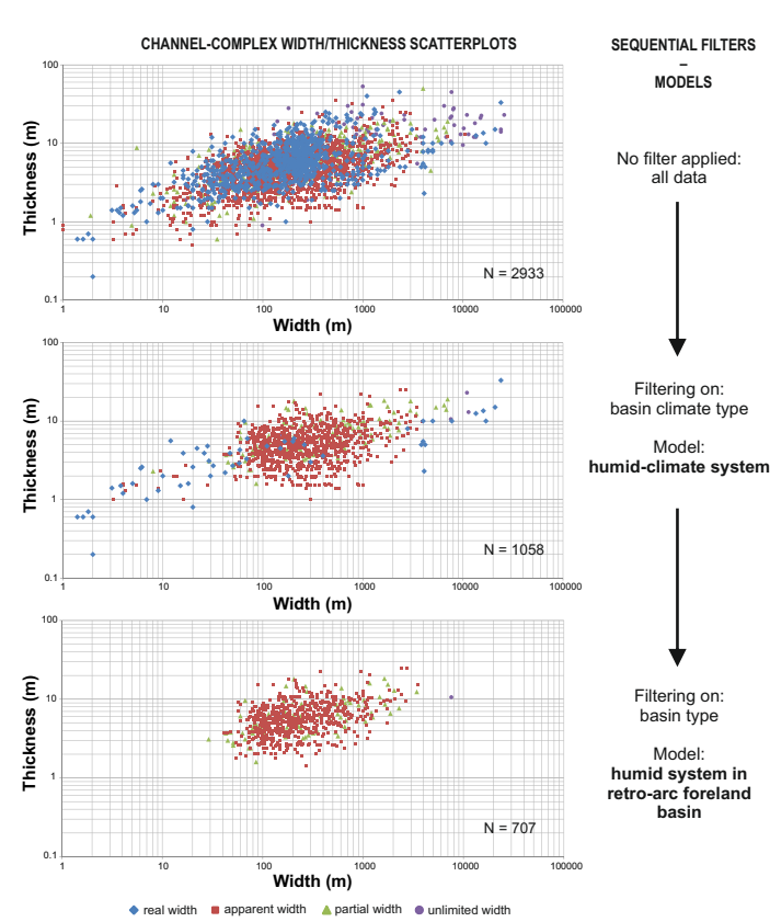
Above. Application of successive filters in FAKTS to examine the width-to-thickness relationships for fluvial successions developed under the influence of humid climatic conditions in retro-arc foreland basins.
