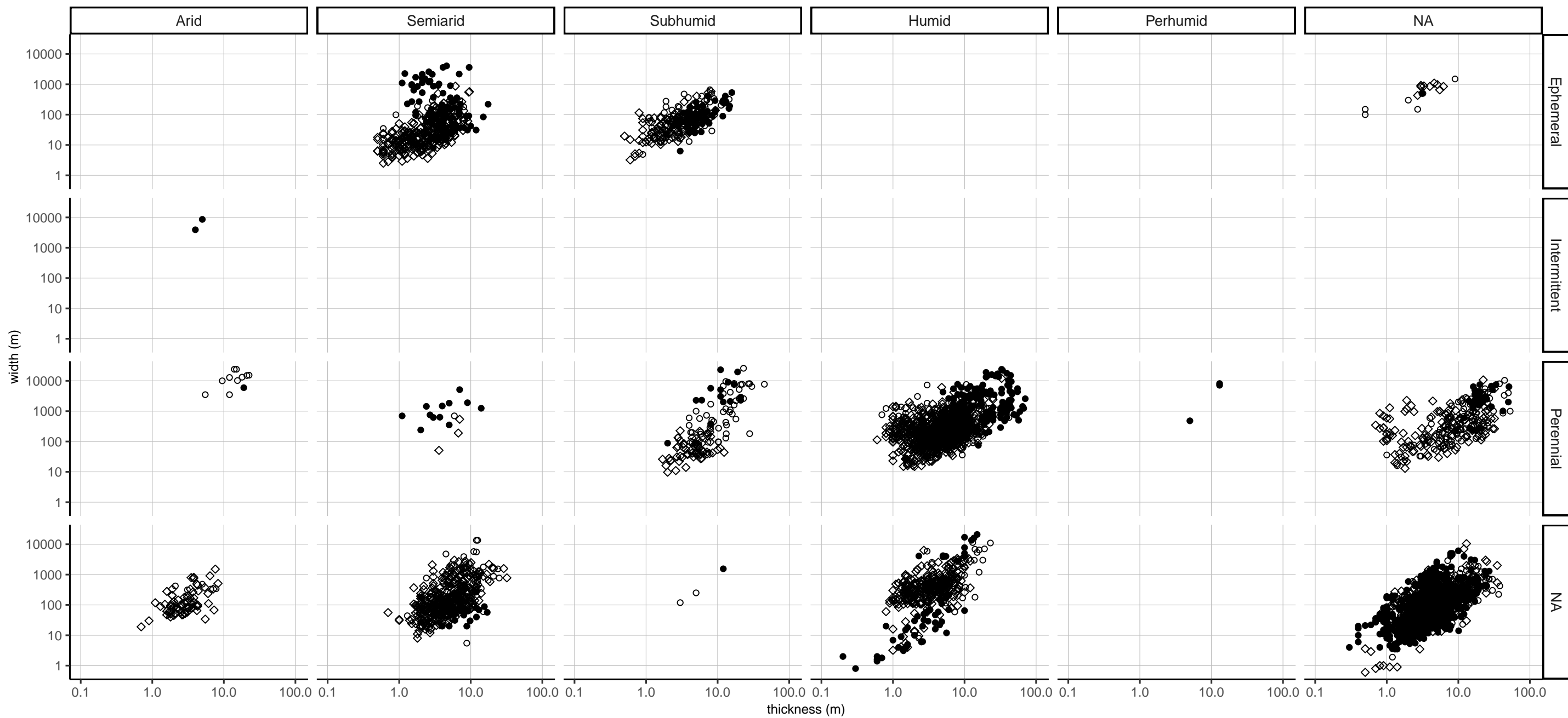
channel-body width vs thickness, by depositional setting, basin climate, discharge regime
