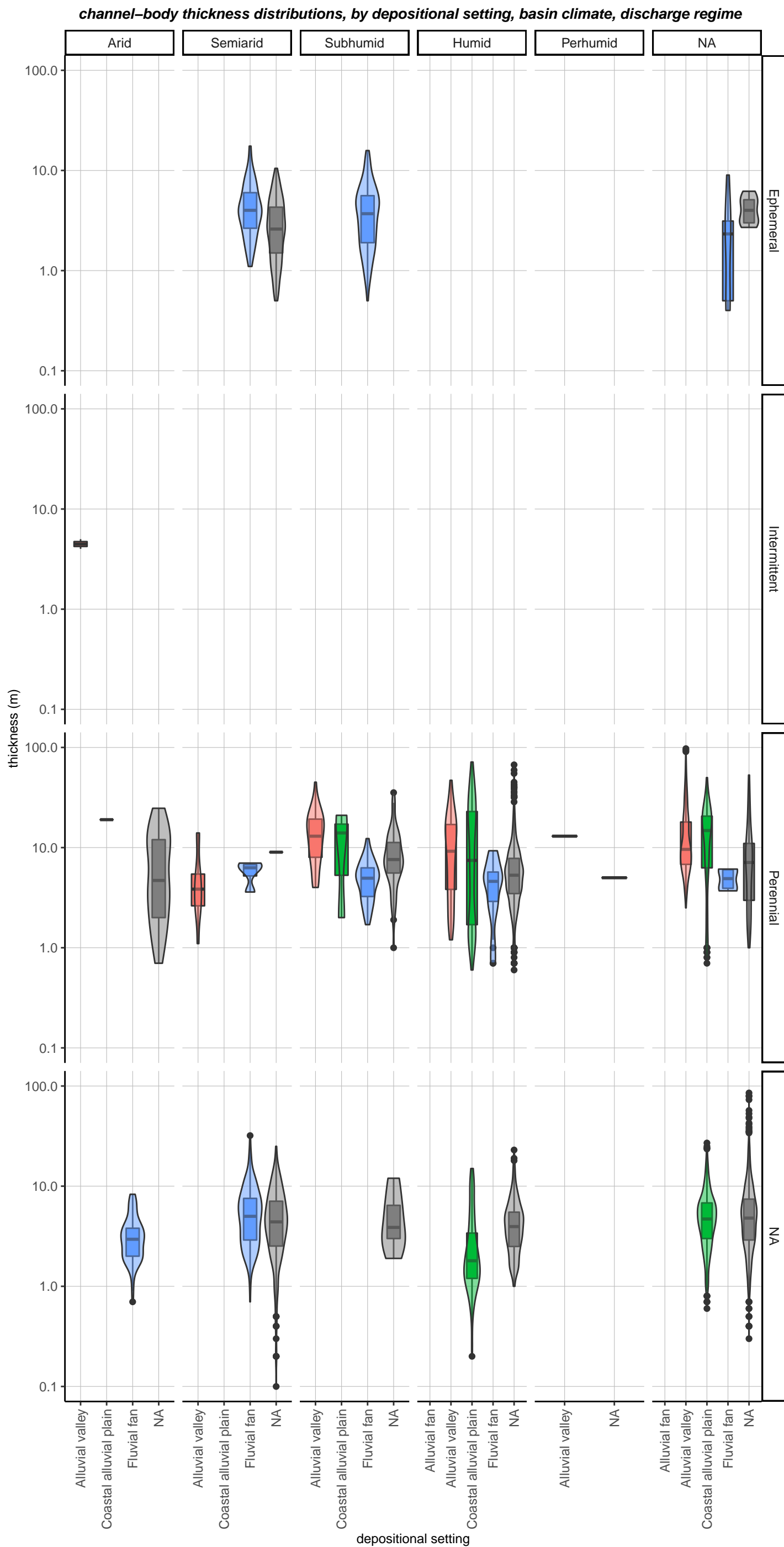
Boxplots and violin plots of thickness distributions of channel bodies for groups of analogues classified on depositional setting and on combinations of river pattern and discharge regime (left) and basin climate and discharge regime (right). Boxes represent interquartile ranges, horizontal bars median values ( n = 6,658 ). NA indicates unclassified analogues
