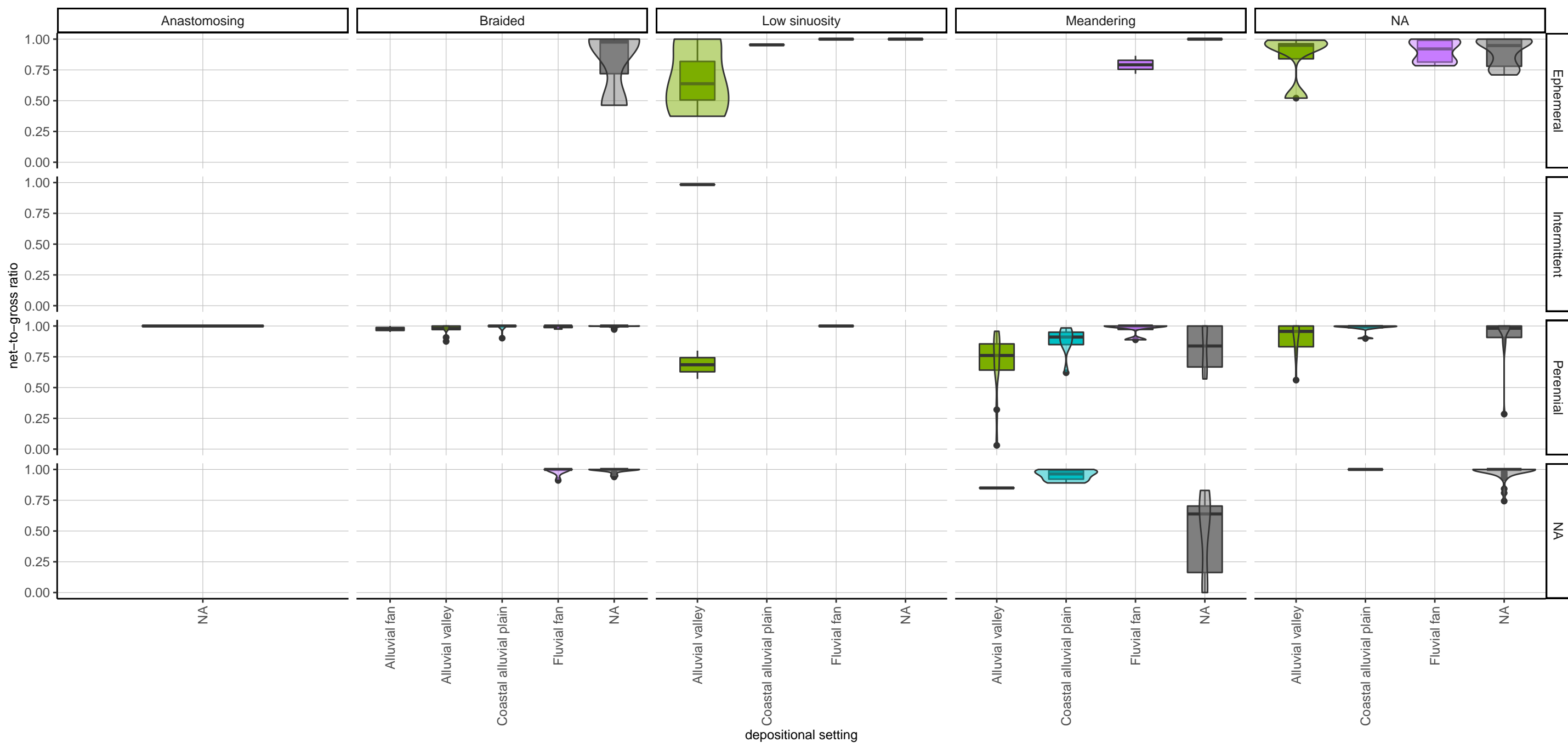
channel-body net-to-gross distributions, by depositional setting, basin climate, discharge regime
