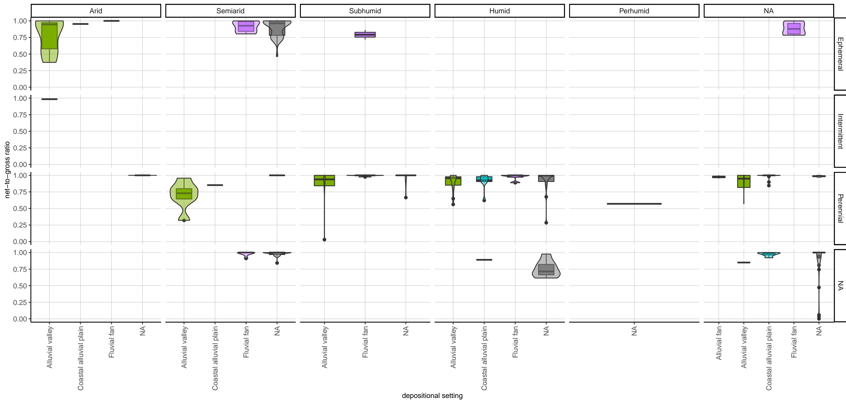
Boxplots and violin plots of distributions of net-to-gross ratios of channel bodies for groups of analogues classified on depositional setting and on combinations of river pattern and discharge regime (top panel) and basin climate and discharge regime (bottom panel). Boxes represent interquartile ranges, horizontal bars median values (n = 239). NA indicates unclassified analogues
